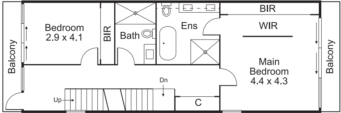
FIRST FLOOR
